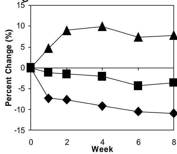
Negative
