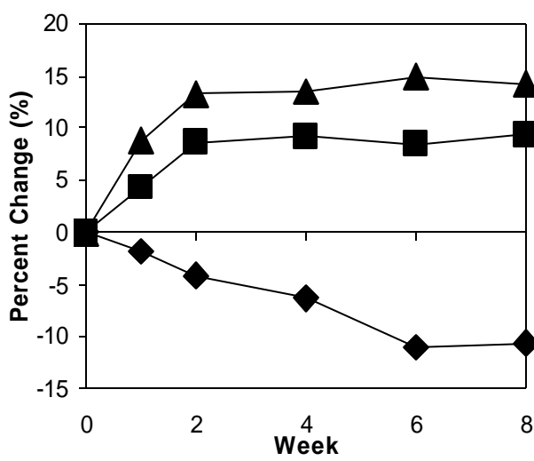
Positive
