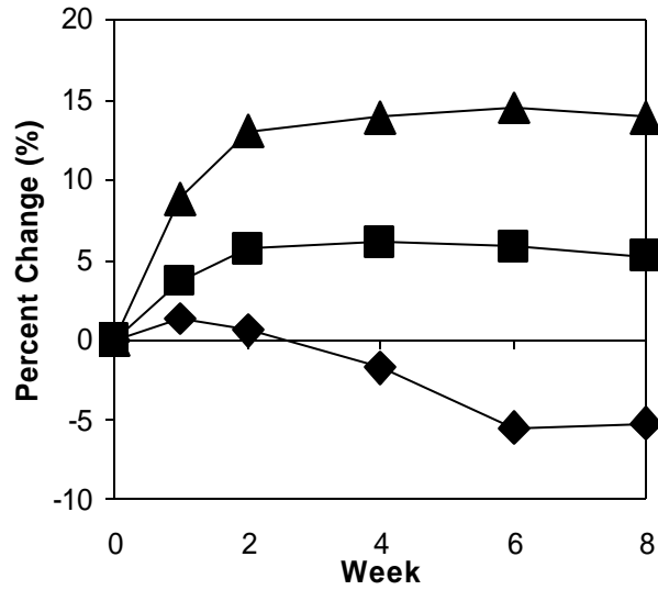
Total Score
